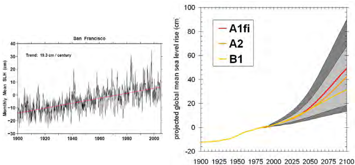
Figure 3. Observed change in sea level rise in San Francisco and projections of global mean sea level rise
