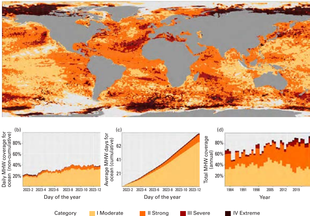
Figure 8. (a) Global map showing the highest marine heatwave category (for definitions, see Data set and methods ) experienced at each pixel over 2023 (reference period 1982–2011). Light grey indicates that no marine heatwave occurred in a pixel over the entire year; (b) Stacked bar plot showing the percentage of the surface of the ocean experiencing a marine heatwave on any given day of the year; (c) Stacked bar plot showing the cumulative number of marine heatwave days averaged over the surface of the ocean, calculated by dividing the cumulative sum of marine heatwave days per pixel weighted by the surface area of those pixels; and (d) Stacked bar plot showing the total percentage of the surface of the ocean that experienced a marine heatwave from 1982 to present. Data are from the National Oceanic and Atmospheric Administration (NOAA) Optimum Interpolation Sea-Surface Temperature (OISST).
