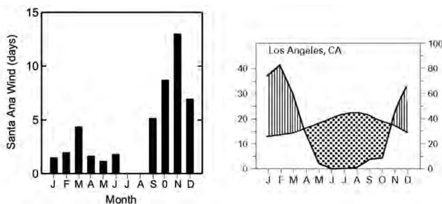
Figure 5. Days of Santa Ana winds (left) and (right) temperature and precipitation in Los Angeles illustrating typical Mediterranean climate of winter rains and summer droughts (from Keeley et al. 2012).
