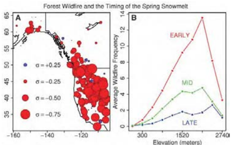
Fig. 2. (A) Pearson’s rank correlation between annual western U.S. large (9400 ha) forest wildfire frequency and streamflow center timing. x axis, longitude; y axis, latitude. (B) Average frequency of western U.S. forest wildfire by elevation and early, mid-, and late snowmelt years from 1970 to 2002. See Fig. 1B for a definition of early, mid-, and late snowmelt years.
