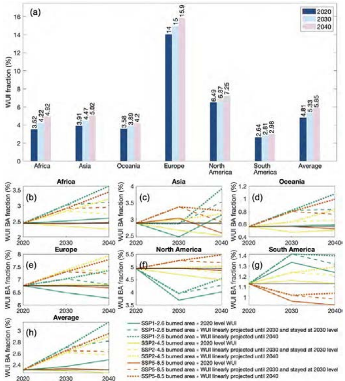
Figure 5. (a) Wildland-urban interface (WUI) fraction (%) in 2020, 2030, and 2040 by continents. (b)–(h) Fraction of burned area within WUI (%) in 2020, 2030, and 2040 under different scenarios. The fraction of burned area within WUI (%) calculated with CESM2 burned area is normalized to the fraction of burned area within WUI (%) in 2020 calculated with MODIS burned area observations (shown in figure 4). An unnormalized version is shown in figure S11.
