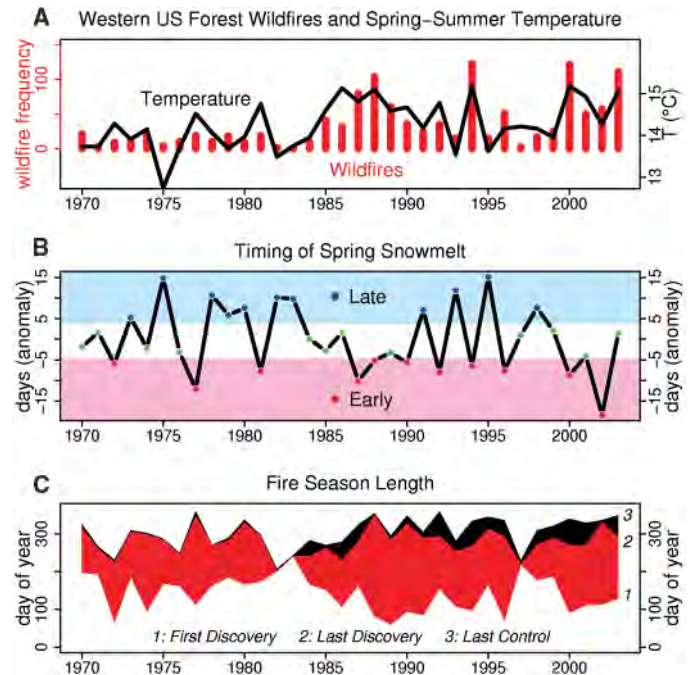
Fig. 1. (A) Annual frequency of large (9400 ha) western U.S. forest wildfires (bars) and mean March through August temperature for the western United States (line) (26, 30). Spearman’s rank correlation between the two series is 0.76 ( P < 0.001 ). Wilcoxon test for change in mean large-forest fire frequency after 1987 was significant ( W = 0.42 ; P < 0.001 ). (B) First principle component of center timing of streamflow in snowmelt dominated streams (line). Low (pink shading), middle (no shading), and high (light blue shading) tercile values indicate early, mid-, and late timing of spring snowmelt, respectively. (C) Annual time between first and last large-fire ignition, and last large-fire control.
