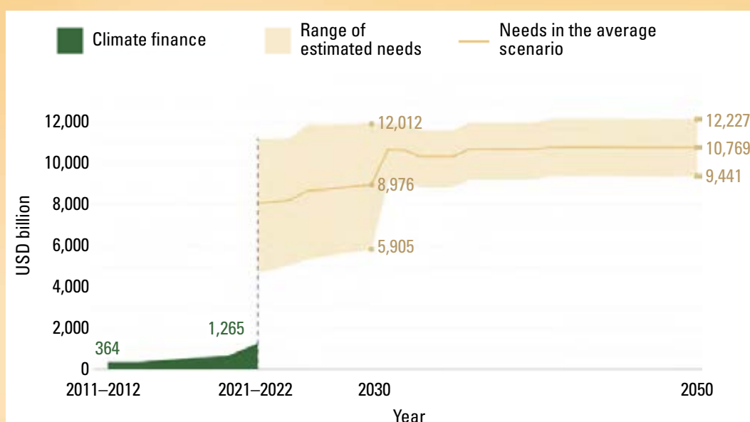
Figure 26. Global tracked climate finance and average estimated annual needs from 2011–2012 through 2050.
